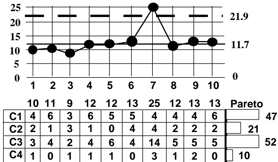
Figure 3 - Shewhart+Pareto charts
