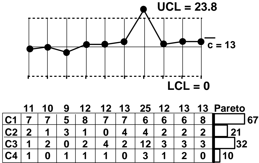
Figure 2 - Shewhart and Pareto charts together
