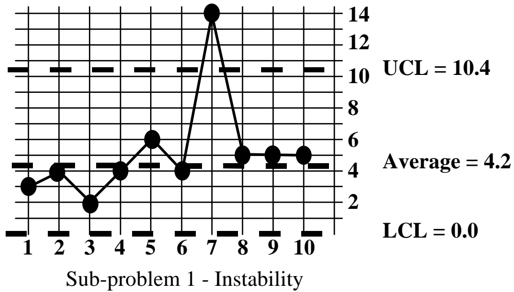
Figure 4 - Category 3 data plotted with instance 7 showing instability
