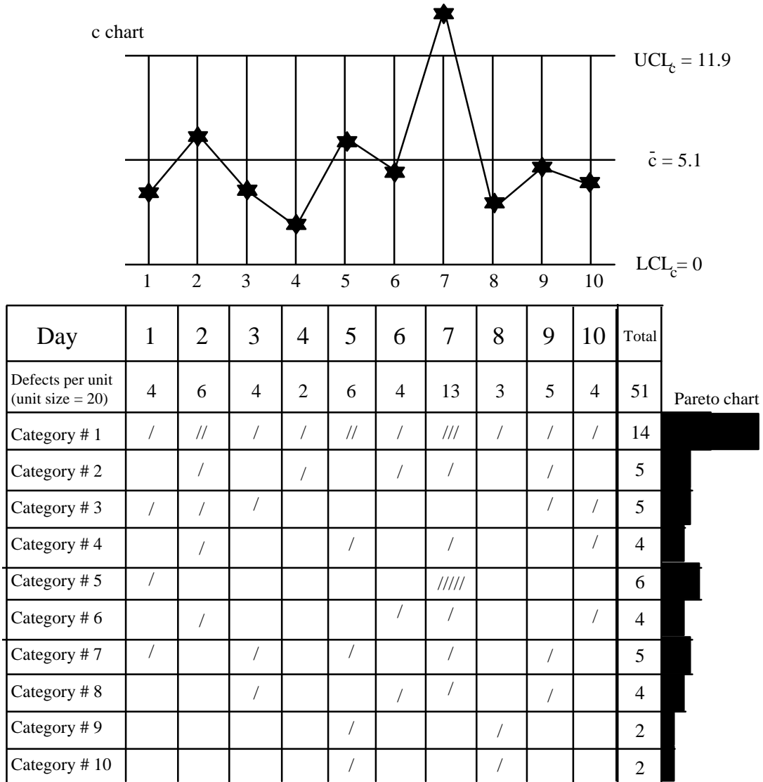
Figure 1 - c+Pareto Chart
